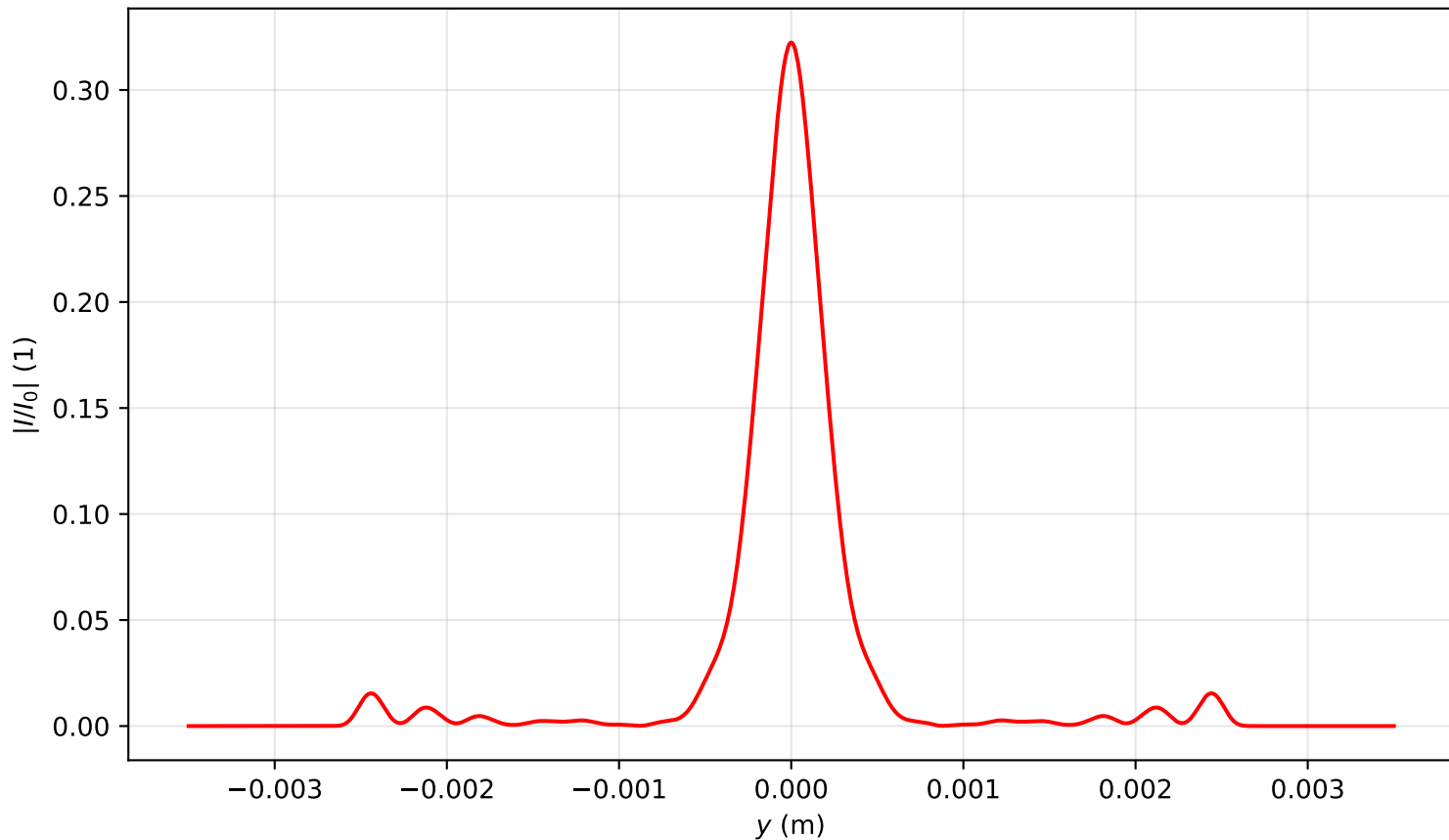
Intensity profile I(x=0, y, z=2.070)/I_0 , P_{in}=6.0P_{cr} , artificial time
